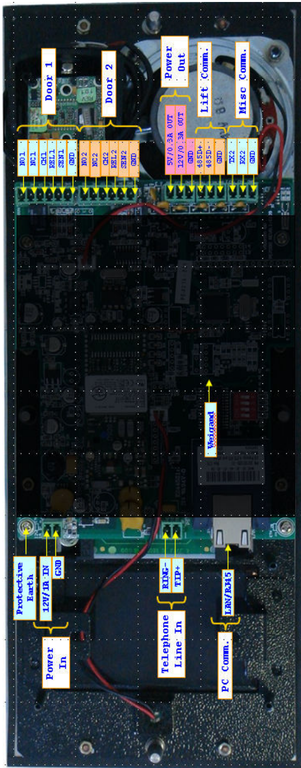
Back View
